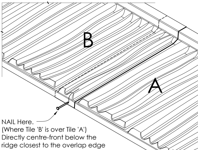
Figure 2.3 Overlap Detail
