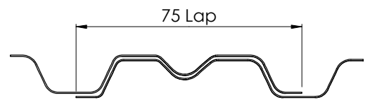
Figure 2.4 Lap Section
