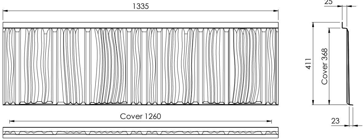
Figure 2.1 Tile Dimensions
