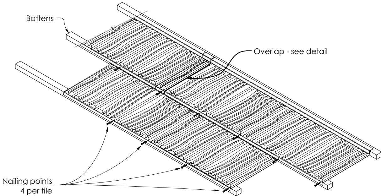
Figure 2.2 Nailing Detail
