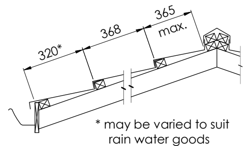
Figure 2.5 Batten Layout
