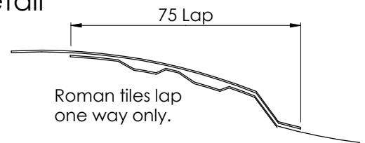
Figure 8.4 Lap Section
