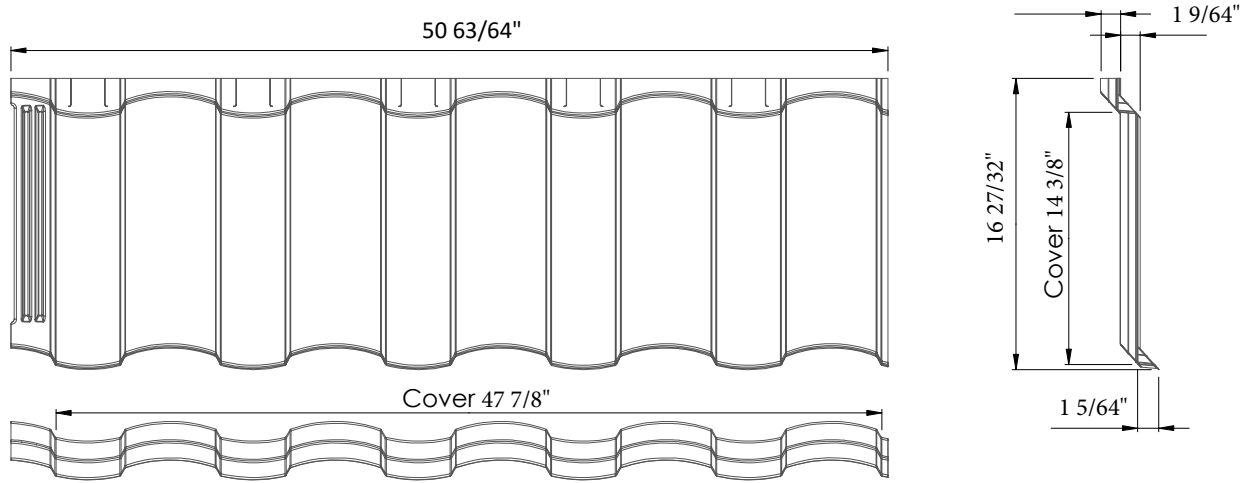
Figure 8.1 Tile Dimensions
