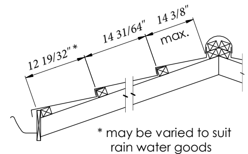
Figure 8.5 Batten Layout
