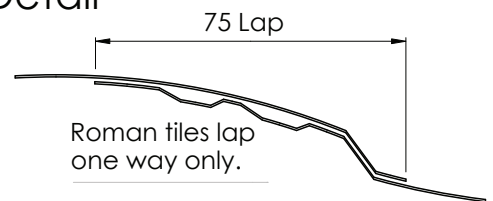
Figure 3.4 Lap Section
