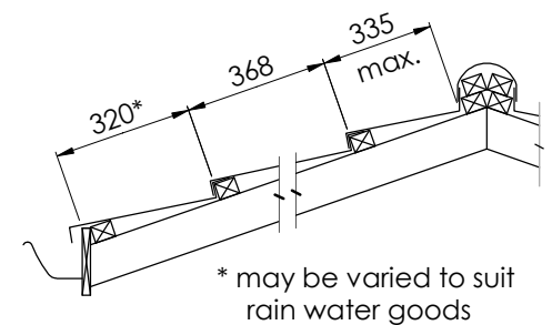
Figure 8.5 Batten Layout
