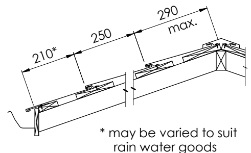
Figure 7.5 Batten Layout
