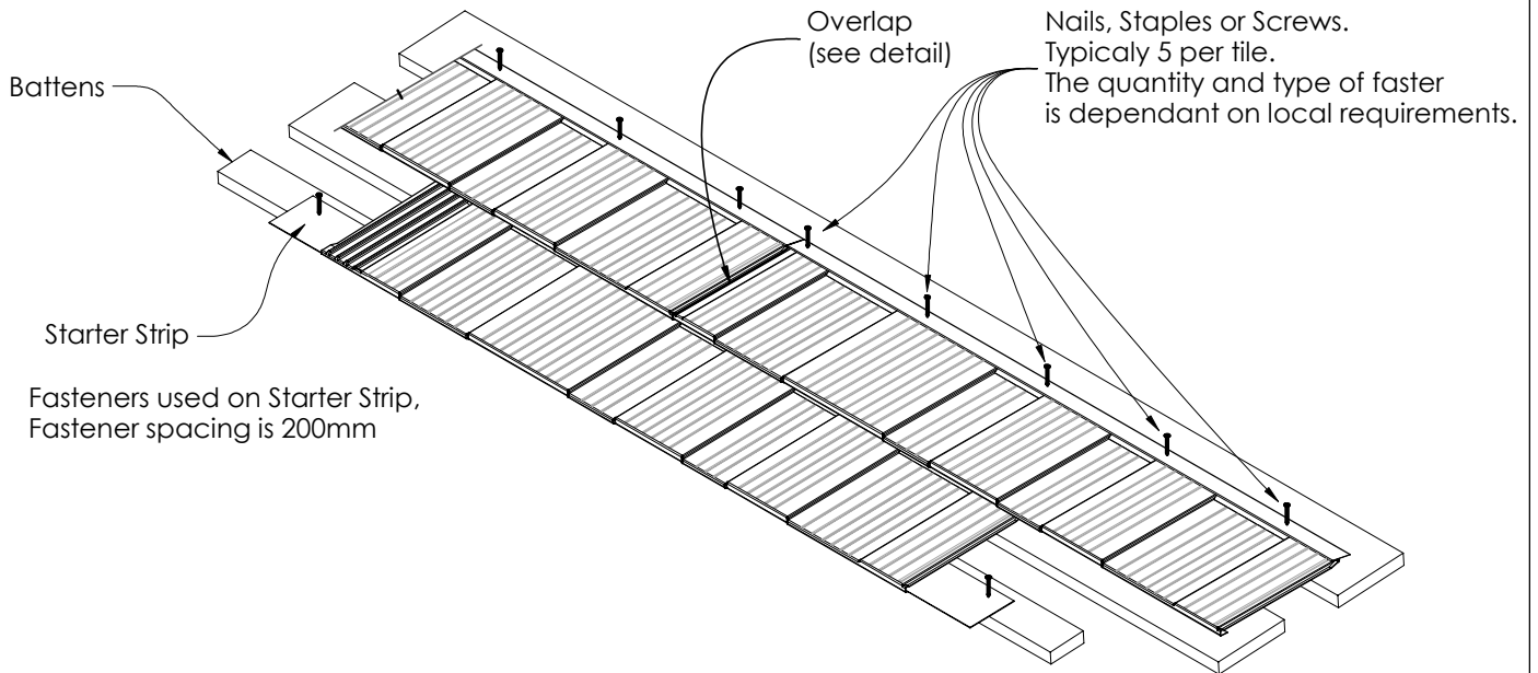
Figure 7.2 Fastening Detail
