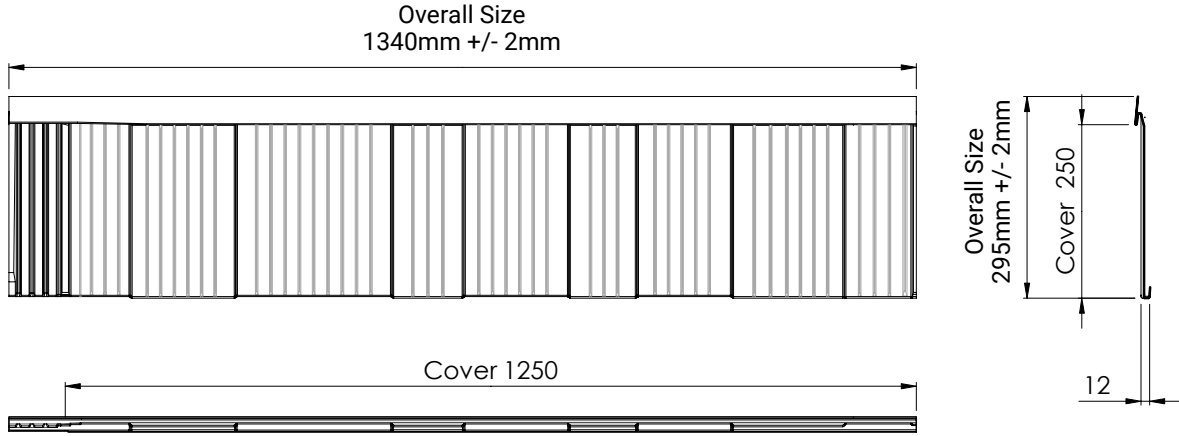
Figure 7.1 Tile Dimensions
