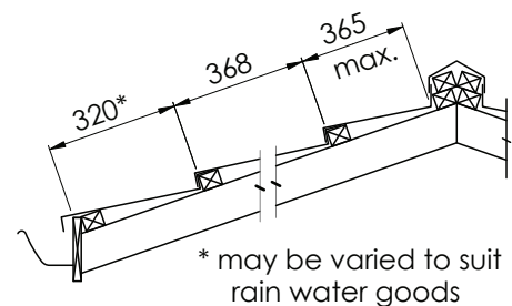
Figure 5.5 Batten Layout
