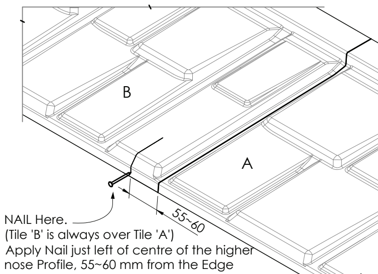
Figure 5.3 Overlap Detail
