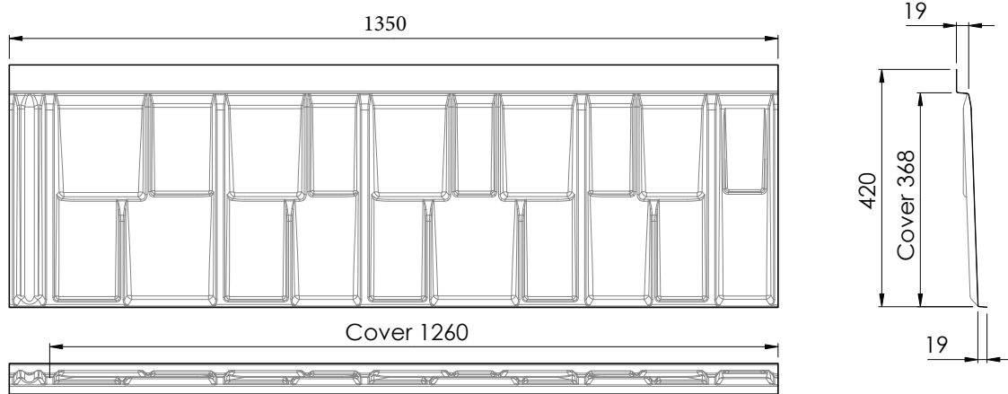
Figure 5.1 Tile Dimensions
